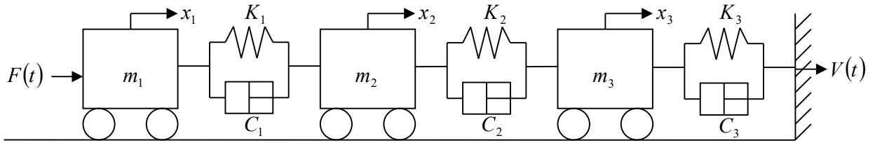
Fig 3.8 Physical model(Spring-Mass-Damper)
